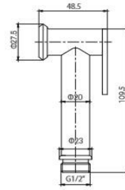
Item No. LST15028 Finish Chrome Material Brass Weight 160g
