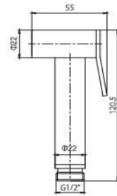
Item No. LST15020 Finish Chrome Material Brass Weight 280g
