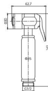
Item No. LST15011 Finish Chrome Material Brass Weight 340g
