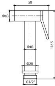
Item No. LST15019 Finish Chrome Material Brass Weight 205g
