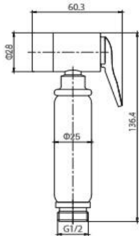
Item No. LST15014 Finish Chrome Material Brass Weight 285g
