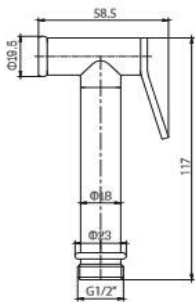
Item No. LST15021 Finish Chrome Material Brass Weight 145g
