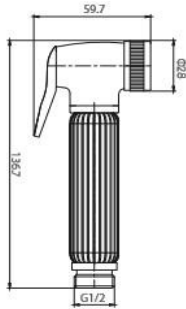
Item No. LST15006 Finish Chrome Material Brass Weight 275g
