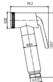
Item No. LST15032 Finish Chrome Material Brass Weight 265g
