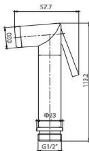
Item No. LST15031 Finish Chrome Material Brass Weight 150g
