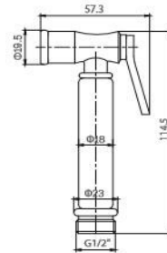
Item No. LST15030 Finish Chrome Material Brass Weight 165g
