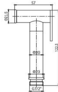
Item No. LST15021A Finish Chrome Material Brass Weight 200g
