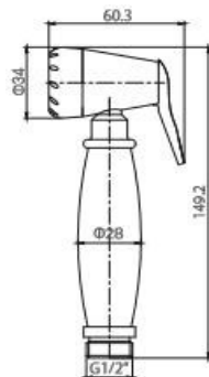
Item No. LST15012 Finish Chrome Material Brass Weight 320g
