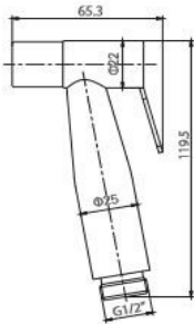
Item No. LST15024 Finish Chrome Material Brass Weight 175g
