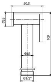
Item No. LST15029 Finish Chrome Material Brass Weight 180g
