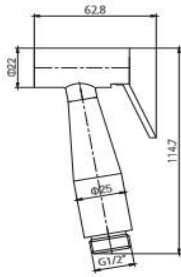
Item No. LST15023 Finish Chrome Material Brass Weight 170g
